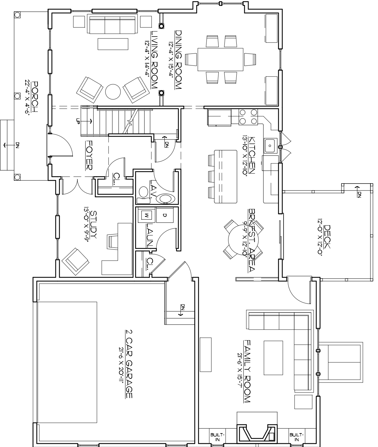
FIRST FLOOR PLAN Scale: 1/8" = 1'-0" 1477 SQ. FT.
